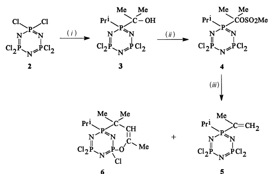
Scheme 1 Reaction scheme for the synthesis of compound 5. (i) \text{MgPr}^i\text{Cl} , [\{\text{CuI}(\text{P}^i\text{Bu}_3)\}_4] then \text{Me}_2\text{CO} ; (ii) \text{ClSO}_2\text{Me} ; (iii) \text{dbu}
