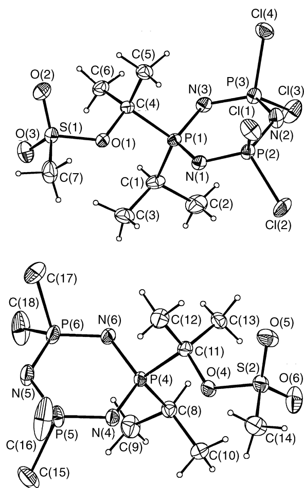
Fig. 2 Perspective ORTEP 30 drawing of the non-hydrogen atoms of compound 4 with the atom labelling scheme for the non-hydrogen atoms. All non-hydrogen atoms are represented by their thermal displacement vibrational ellipsoids drawn to encompass 50% of the electron density; the hydrogen atoms are drawn with an arbitrary radius
